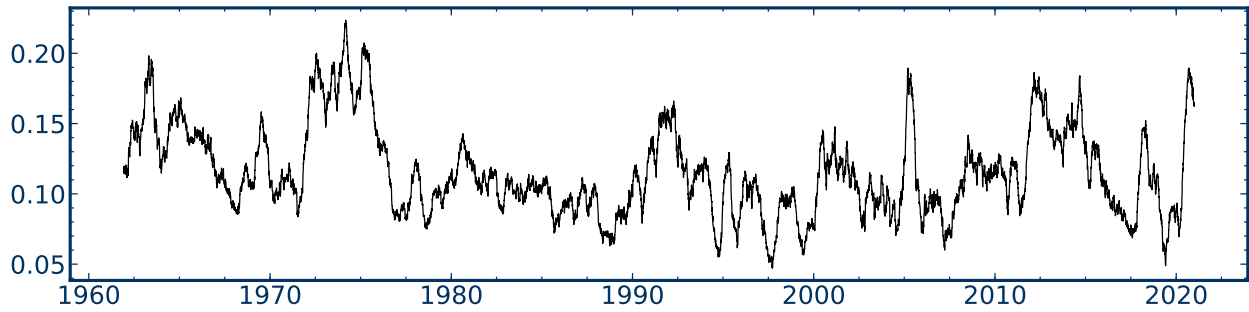
(b) Treasury Market Complexity measure (T-COM)
