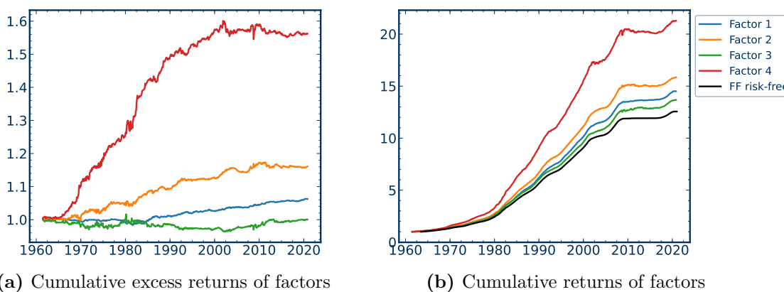
Figure IA.10: Cumulative excess returns and returns of the first four KR factors
