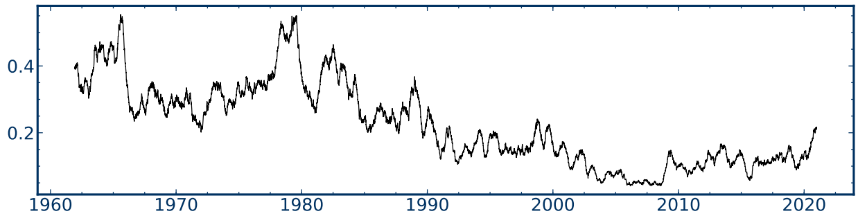
(a) Idiosyncratic Treasury Volatility measure (IT-VOL)
