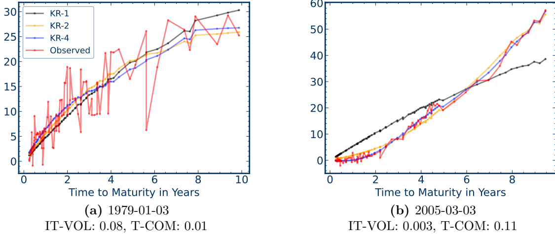
Figure 17: Market Conditions on Example Days
