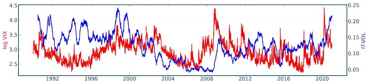
Figure A.10: IT-VOL and VIX
